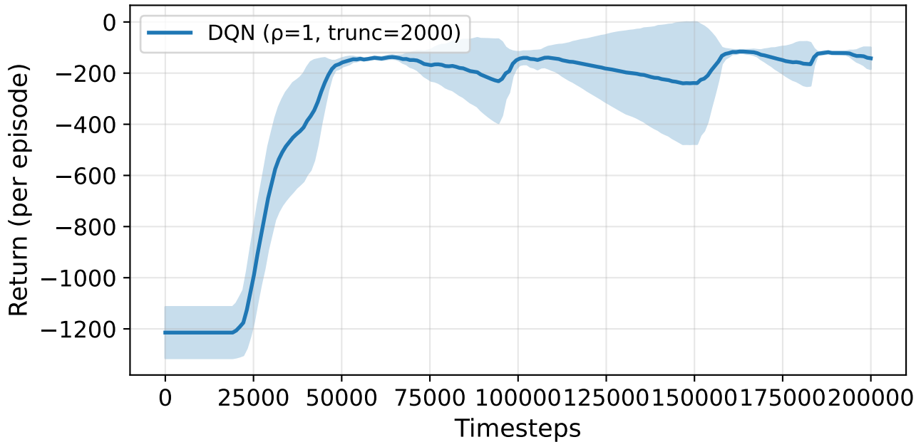
Vanilla DQN on MountainCar-v0 (mean \pm 95% CI, 15 seeds)
